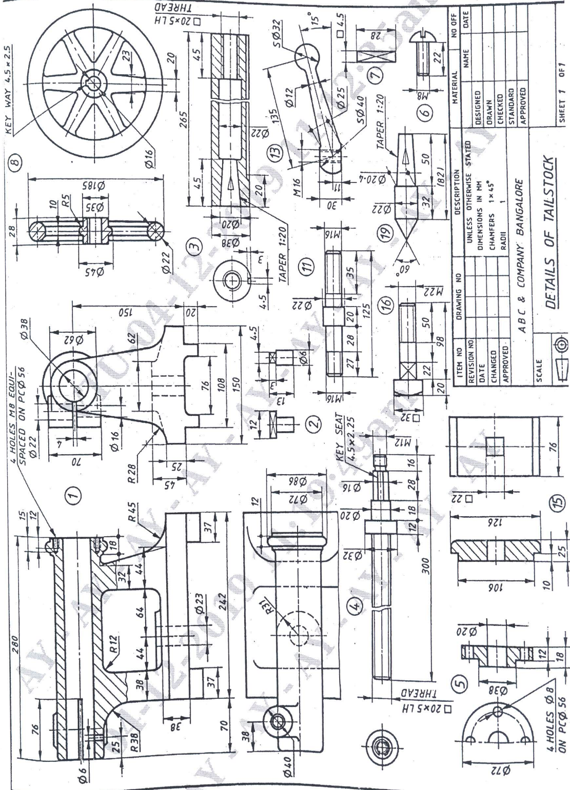
Figure 2: Details of Tail Stock
