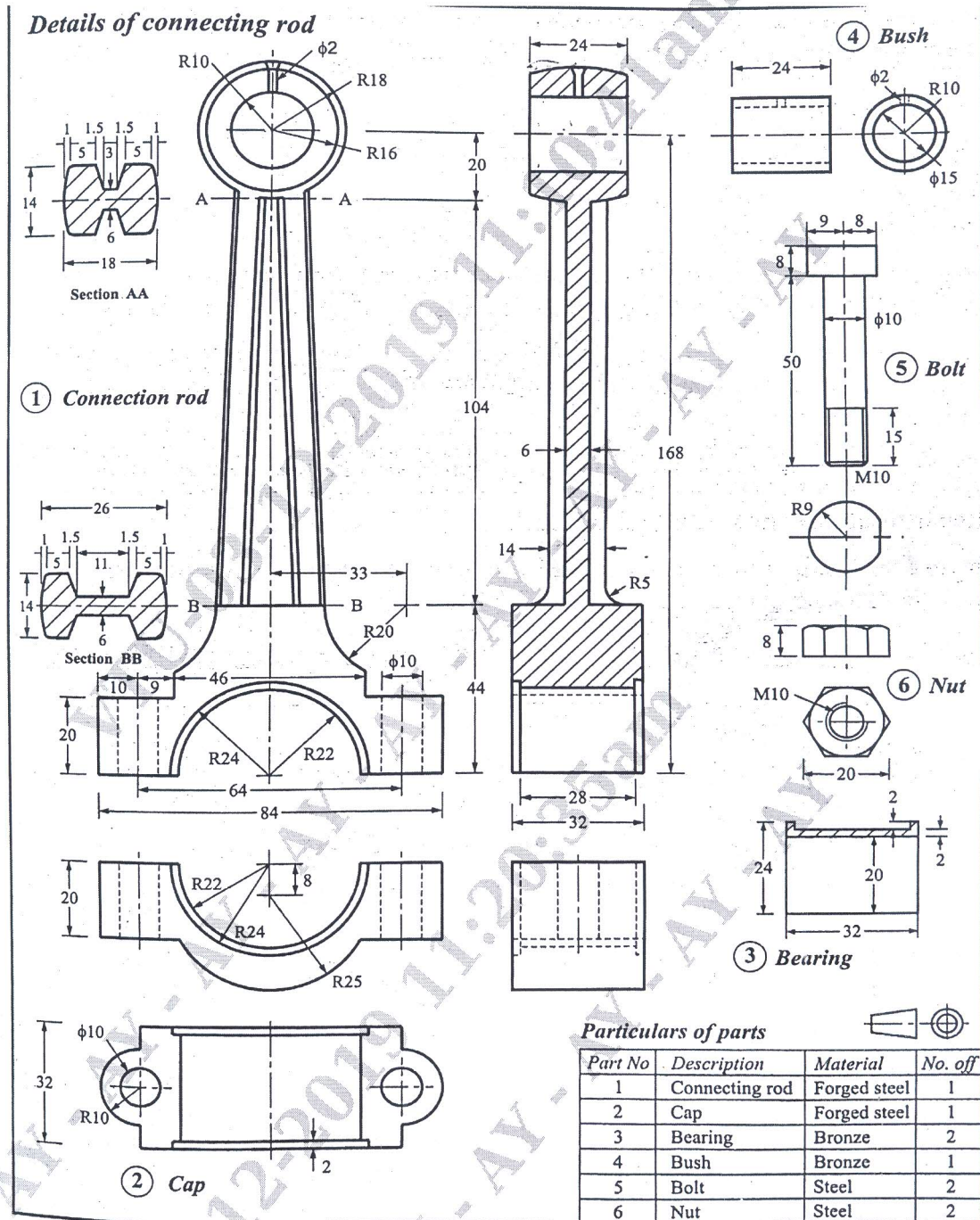
Figure 2: Details of Connecting rod
