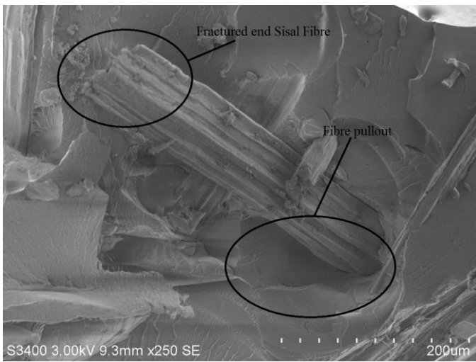
Figure 6 SEM image of Tensile Failure 6% treated 5 mm Sample
