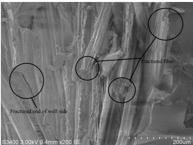
Figure 7 SEM image of Flexural Failure 6% treated 3mm Sample
