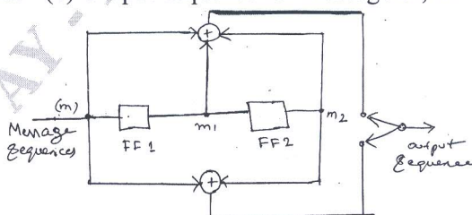
Convolutional encoder
