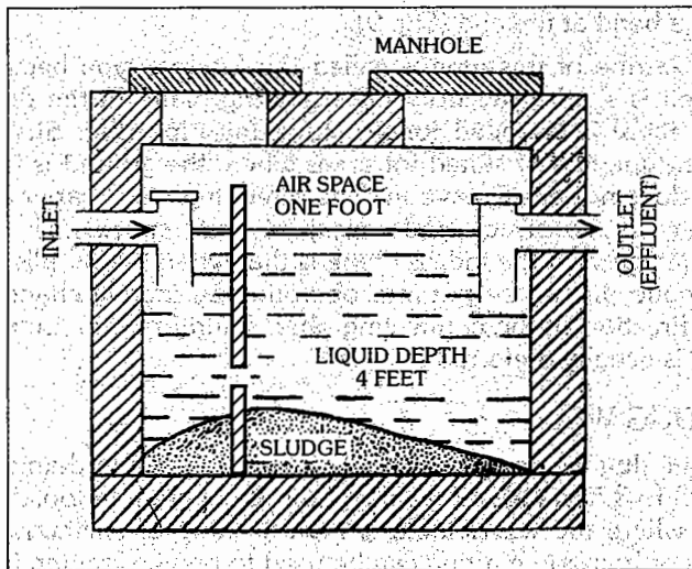
FIG. 10 Septic tank
